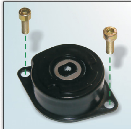
Image 2: Design with two M8x22 bolts
