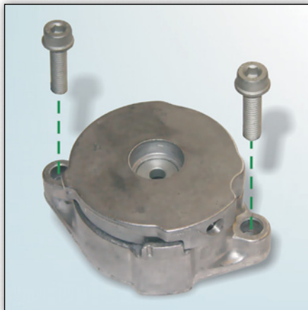
Image 1: INA design with two M8x35 bolts
